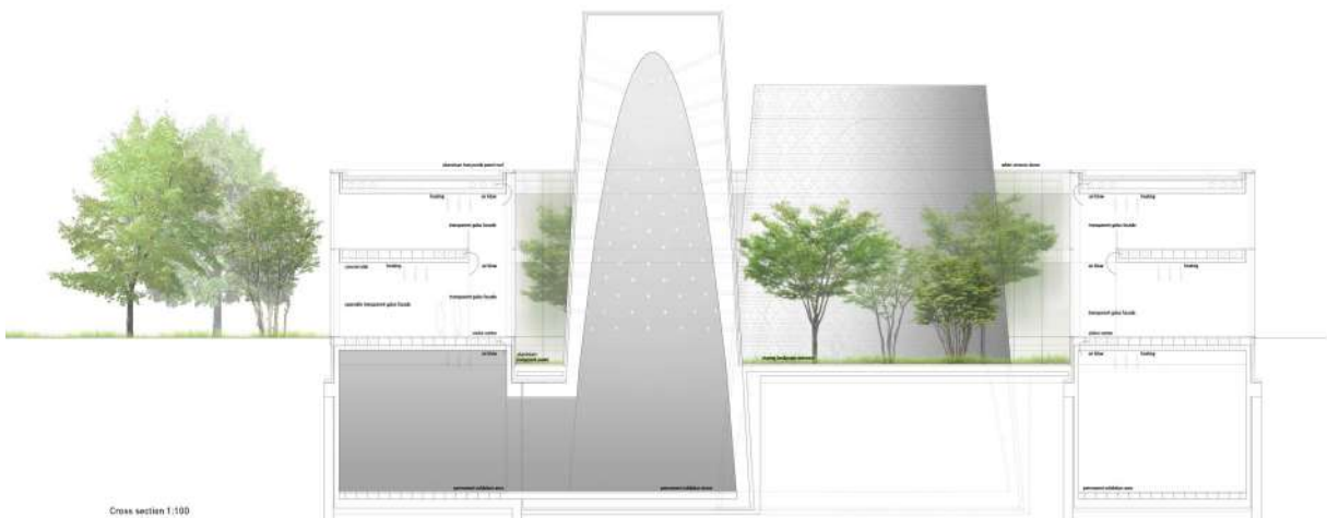
Cross section 1:100
